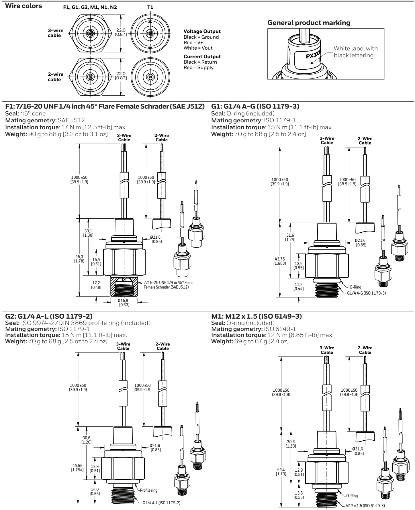
Figure 8. Cable Harness Mounting Dimensions (For reference only. mm/[in].)
