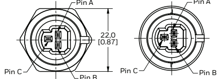
Figure 6. Metri-Pack Mounting Dimensions (For reference only. mm/[in].)
