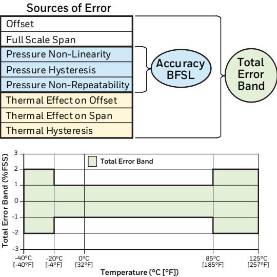
Figure 1. TEB Definition and Temperature Performance
