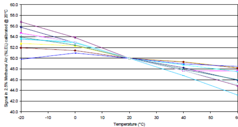
Effect of Temperature on Methane Signal
