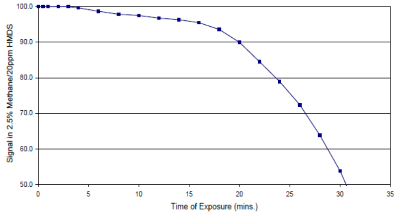
Accelerated Life Tests 4P-90 - HMDS Poison Resistance
