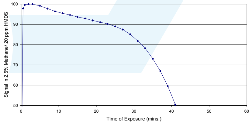
Accelerated Life Tests 4P-75 HMDS Poison Resistance
