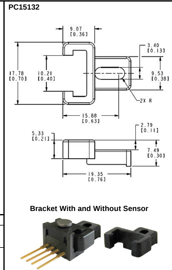
Figure 3. Plastic Mounting Bracket Mounting Dimensions (For reference only: mm/[in.])
