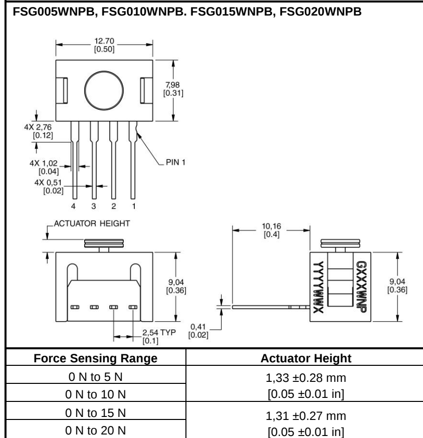
Figure 2. Sensor Mounting Dimensions (For reference only: mm/[in.])
