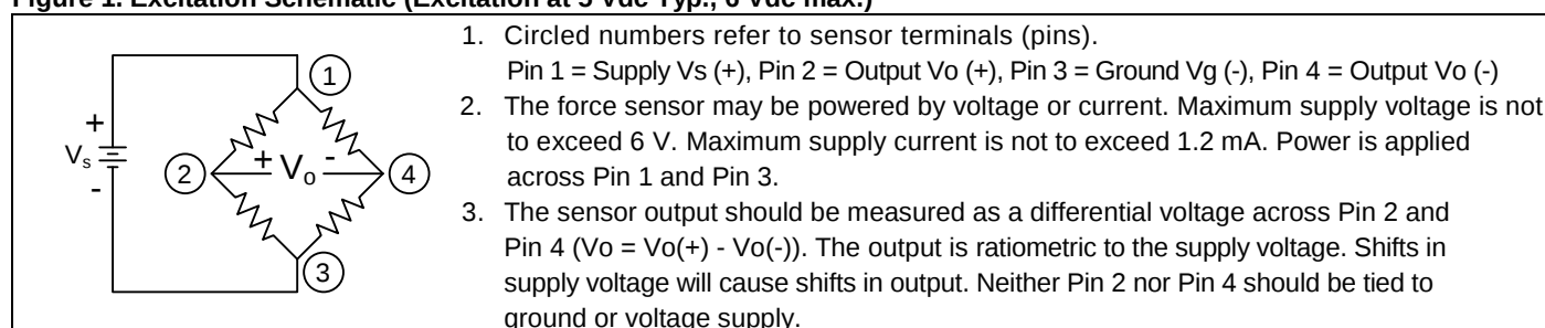
Figure 1. Excitation Schematic (Excitation at 5 Vdc Typ., 6 Vdc max.)
